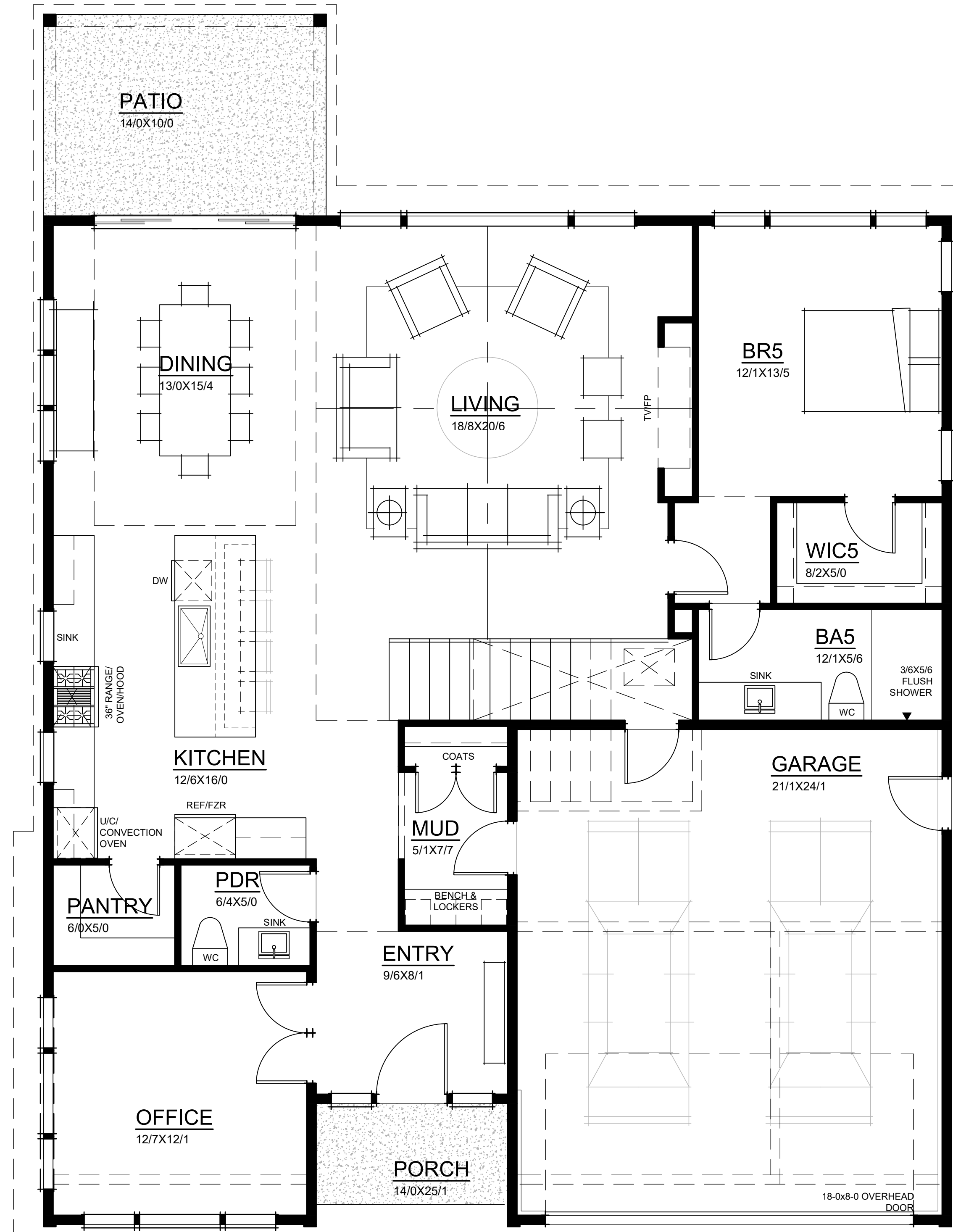
FINN HILL - HIPPED ROOF MAIN FLOOR PLAN
