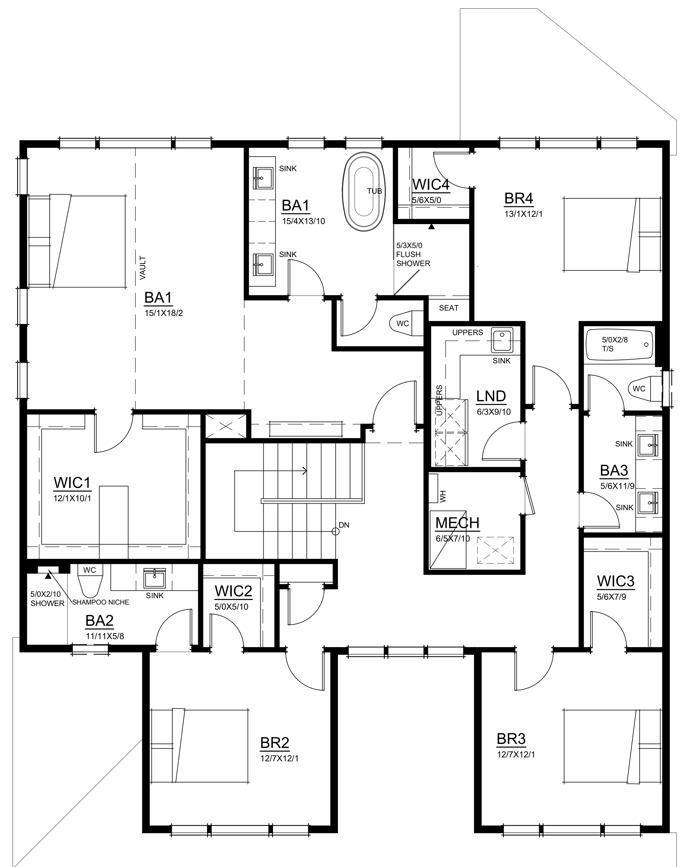
FINN HILL - GABLED ROOF UPPER FLOOR PLAN
