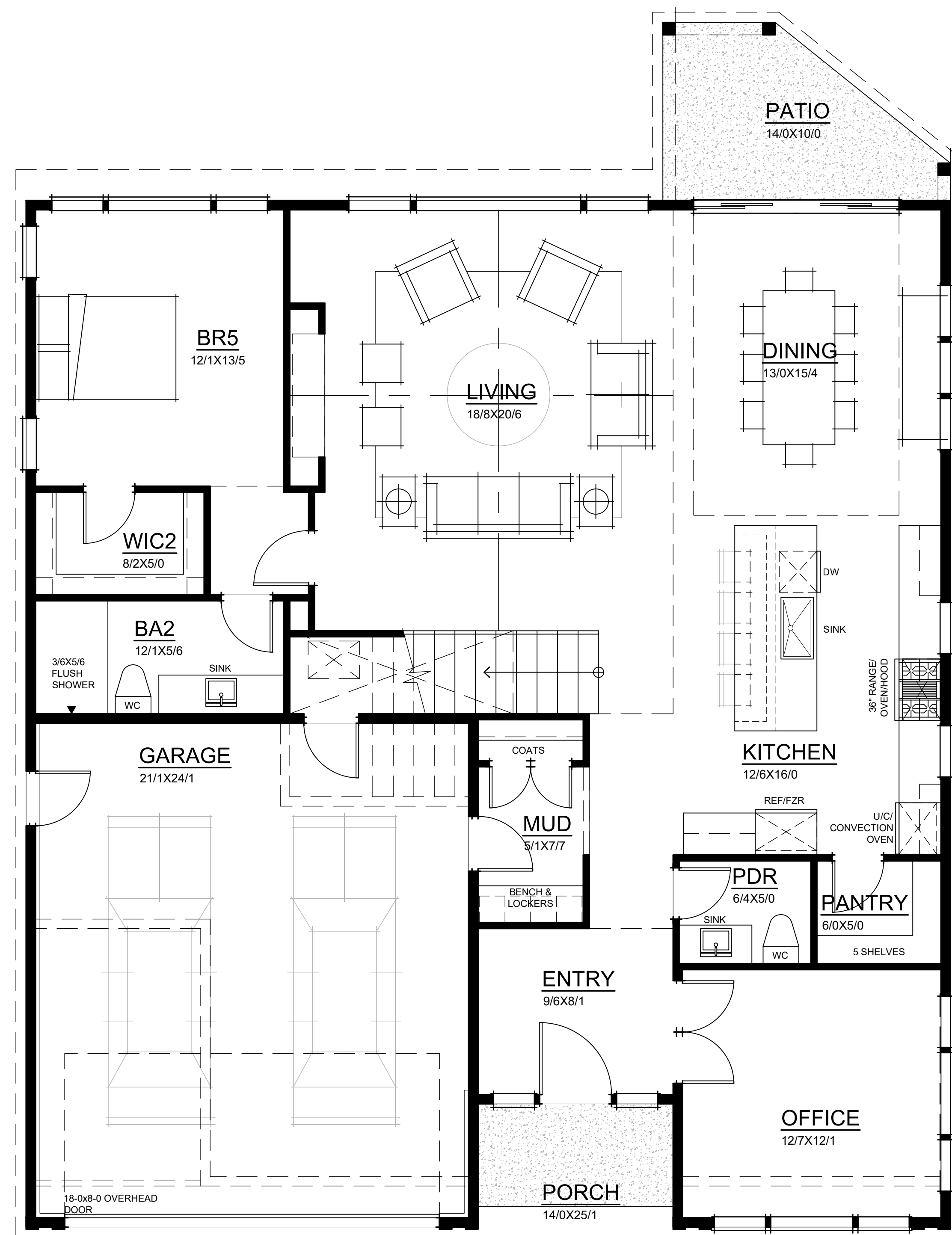
FINN HILL - GABLED ROOF MAIN FLOOR PLAN
